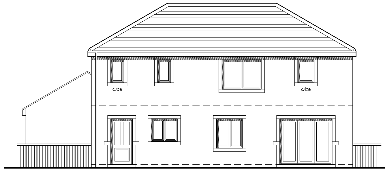
Rear Elevation
